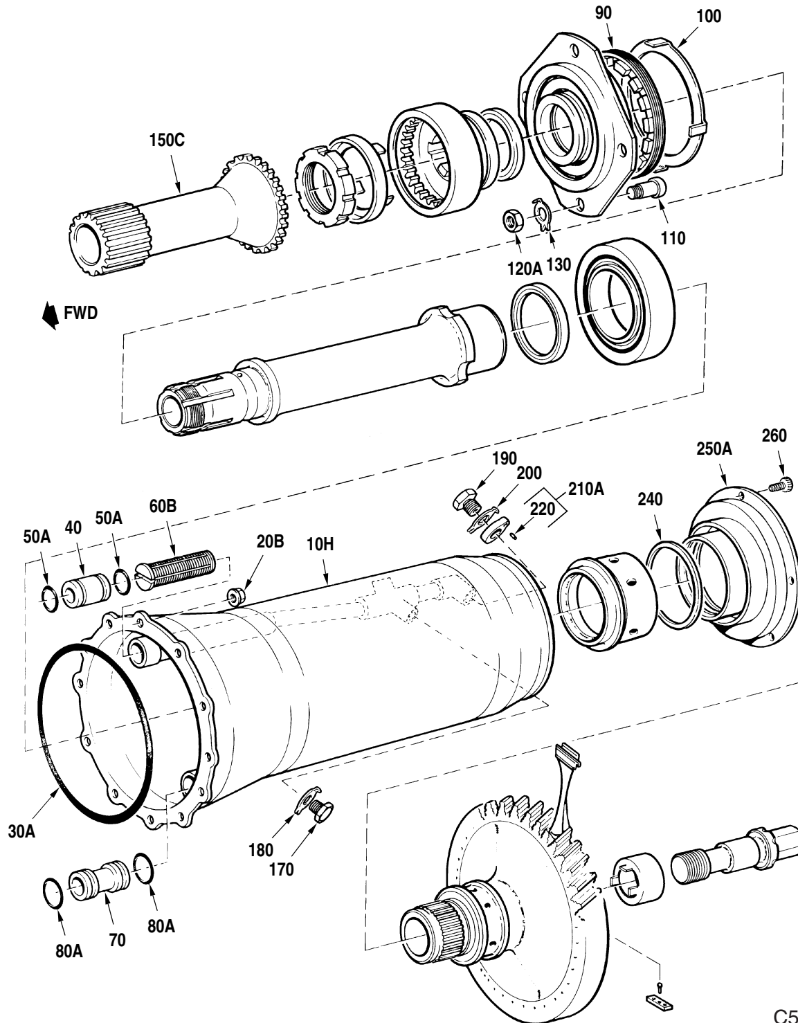
Power Turbine Installation (Pre-SB1057) Figure 1
